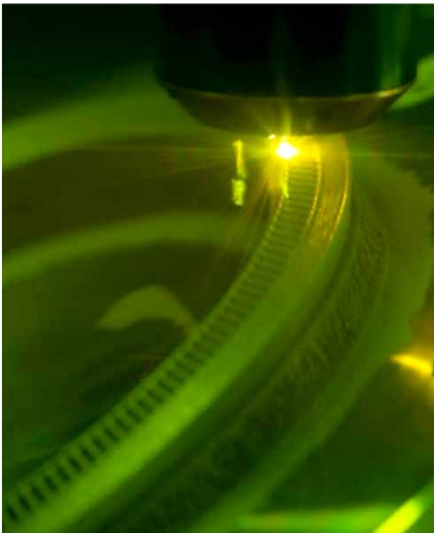
In-process image of laser blown powder directed energy deposition. (Courtesy: RPM Innovations, Inc.)
